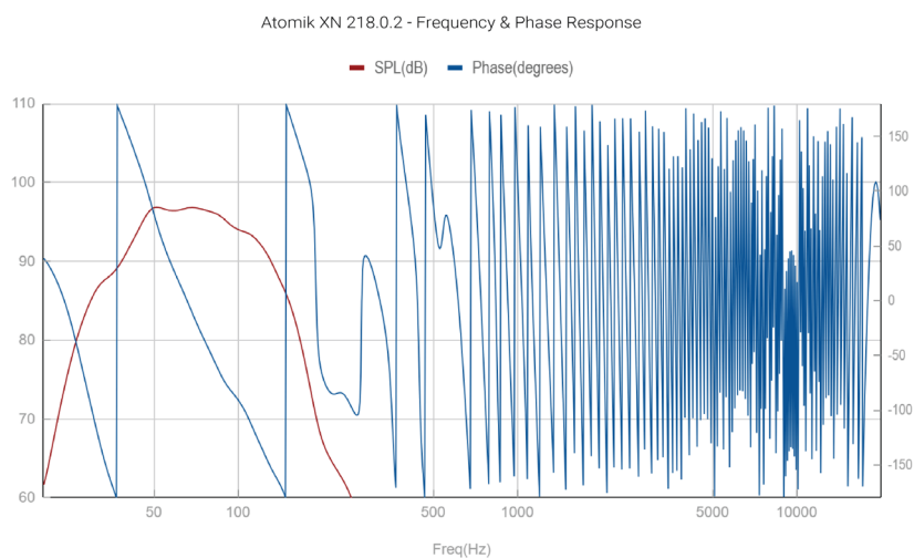
Frequency & Phase Response - Processed
